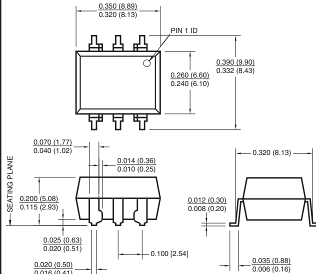
Package Dimensions (Surface Mount)
